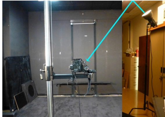
Figure 10. The University of Kansas Spencer Museum of Art digitization lab setup for oversized materials.
